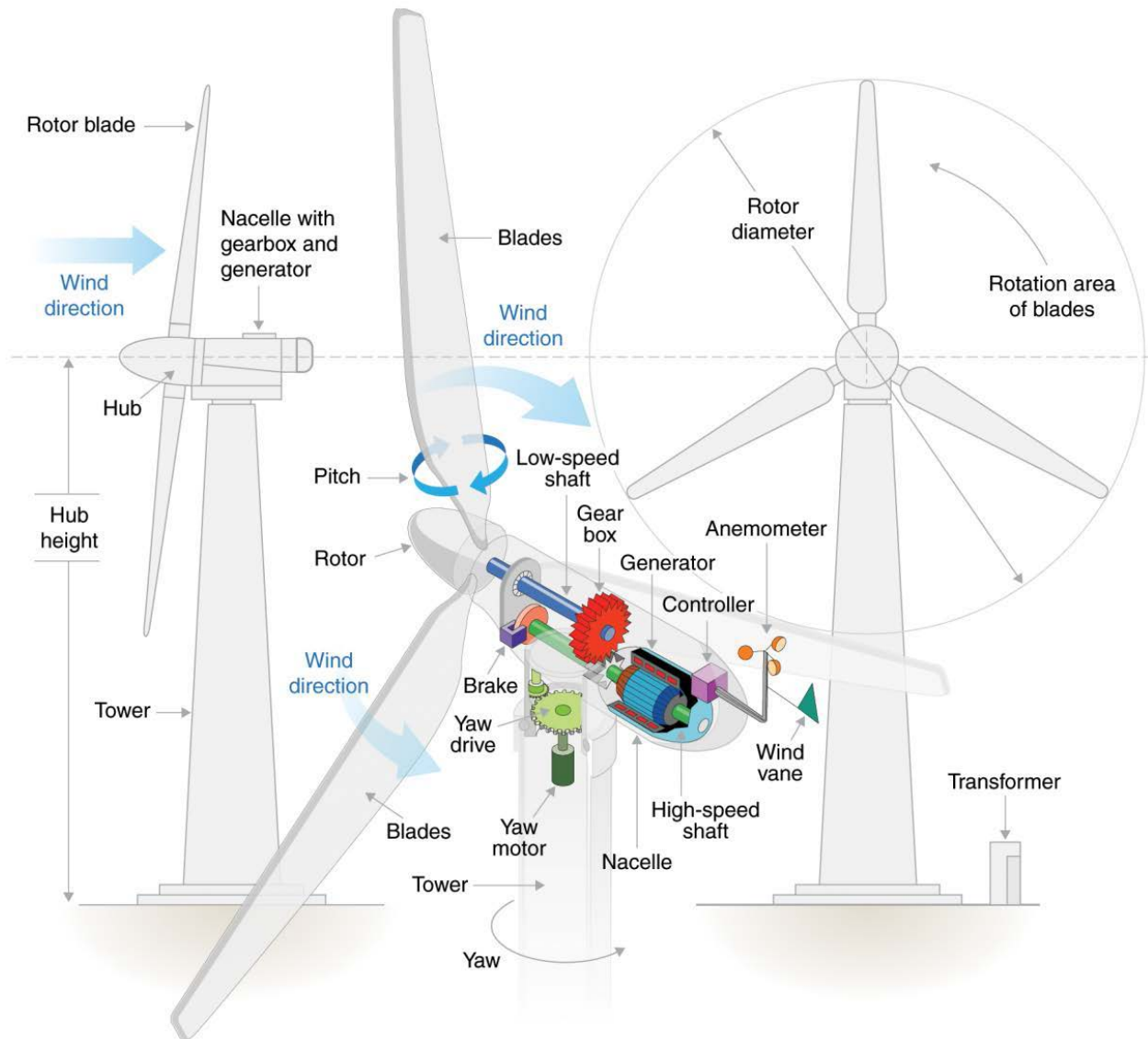
Figure 2.10.1-1. Components of a wind turbine. Source: Augustine (2012).
