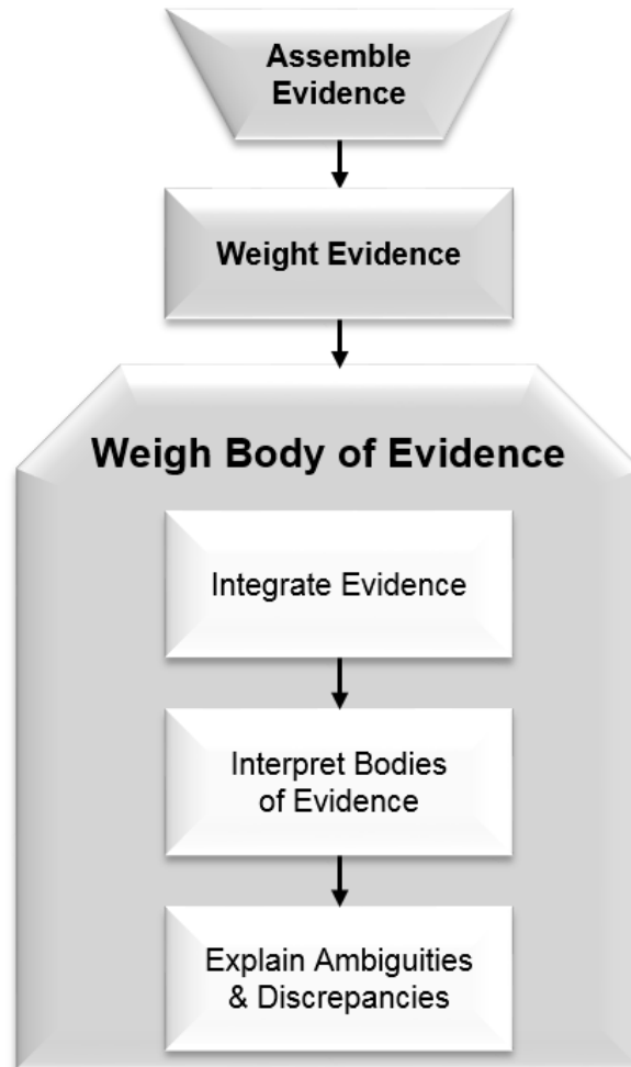
Figure 6-1. An elaboration of the process for weighing the body of evidence, the third step in weight of evidence.
