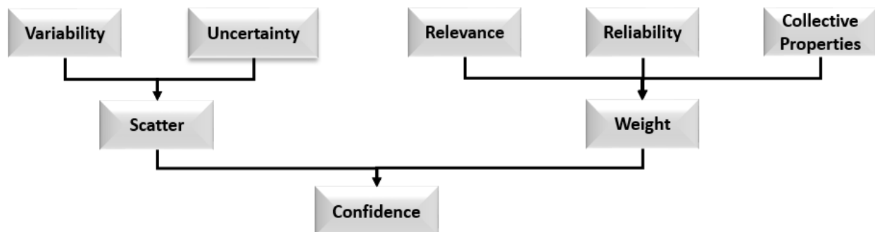
Figure 9-1. A diagram of the combination of statistical scatter and qualitative weight to define the confidence that should be afforded an assessment result.
