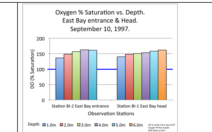
Figure 5-10. Dissolved oxygen saturation levels vs. depth, BISS stations BI-2 and BI-1 (East Bay). September 10, 1997. Blue line shows 100% saturation. Percent saturations calculated via USGS DO TABLES tool from observed water salinity and temperature data from BISS spreadsheet.
