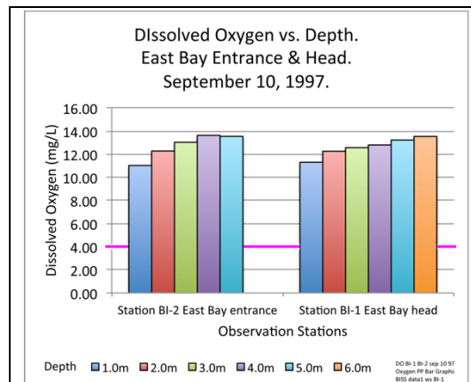
Figure 5-9. Dissolved oxygen concentrations vs. depth, BISS stations BI-2 and BI-1 (East Bay). September 10, 1997. Red line shows 4.0 mg/L ecological stress threshold. The water quality standard here is 5.0 mg/L. Data Source: BISS spreadsheet.
