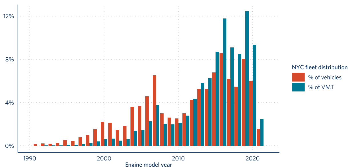
Figure A1. Fleet model year distribution based on vehicle registrations in New York City and estimated share of total VMT.
