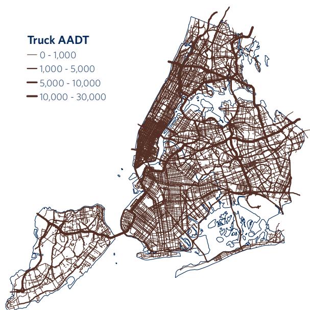
Figure A4. Spatial truck activity data.
