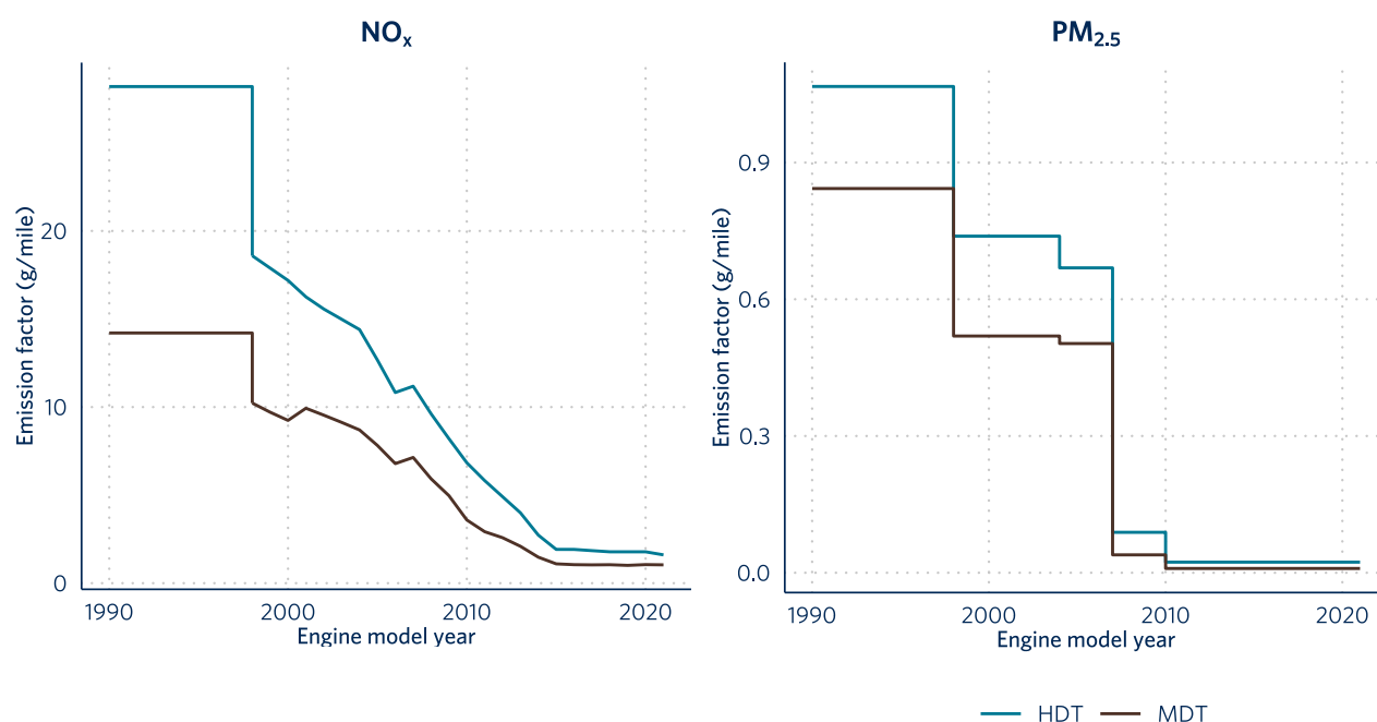
Figure A2. NO x and PM 2.5 emission factors by engine model year.
