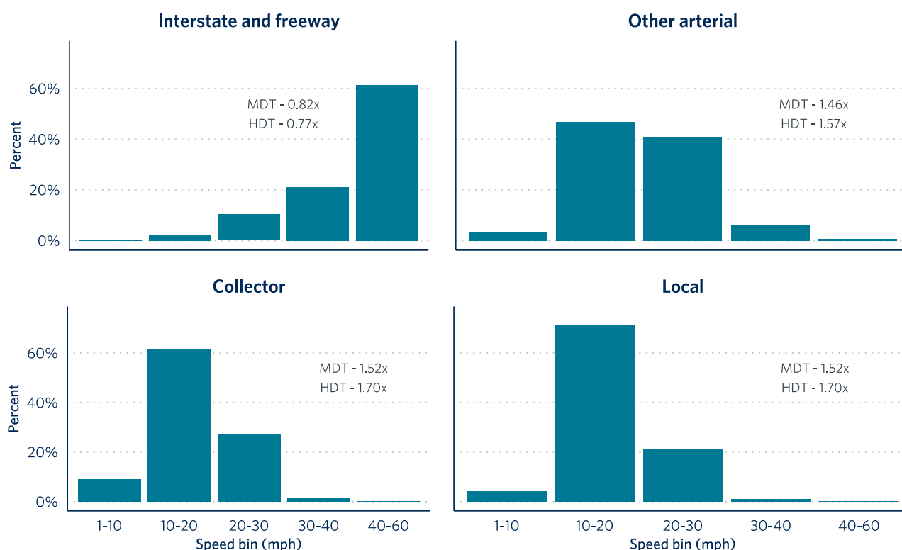
Figure A3. Distribution of activity by speed bin for each road type and average emission factor multipliers for speed adjustment.
