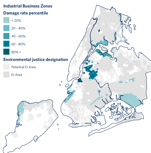
Figure 9. Damage rates by industrial business zones (IBZs) and environmental justice areas.
