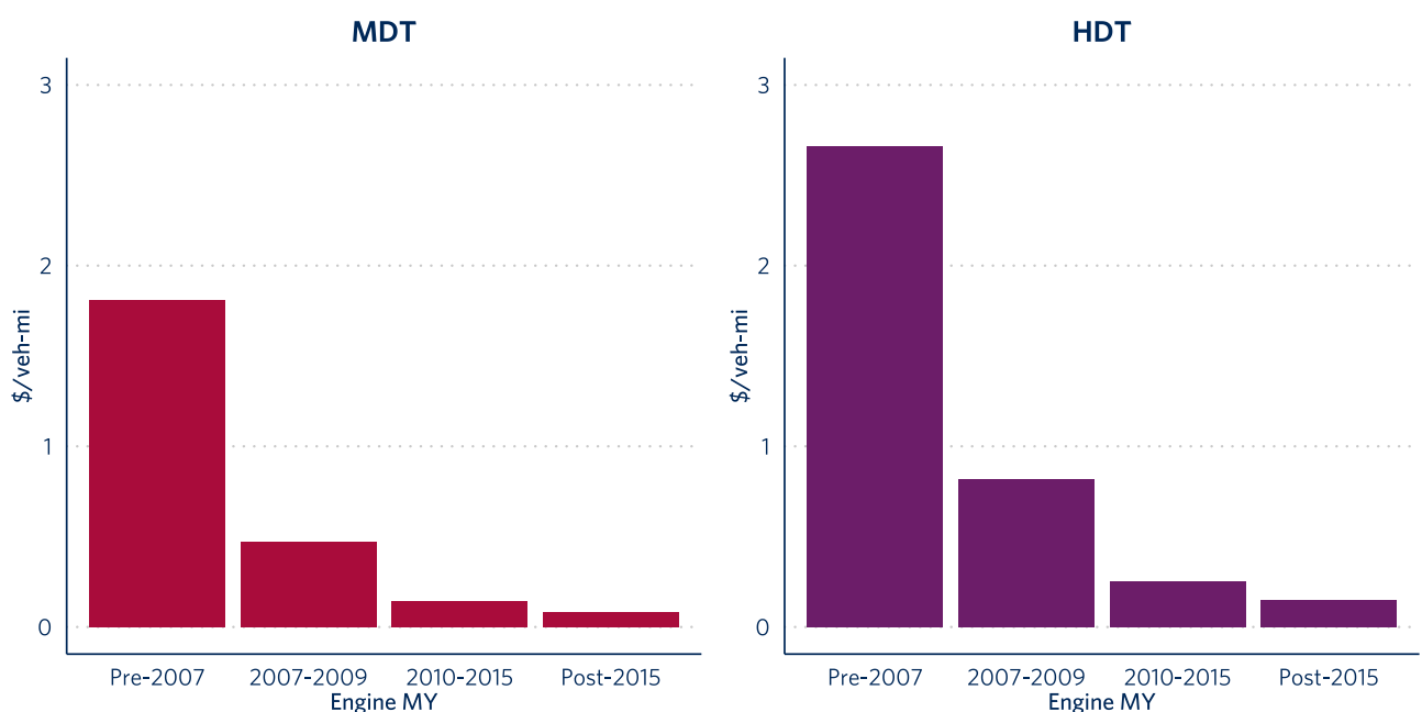
Figure ES-1. Mortality-based damages of diesel trucks operating in New York City by engine model year (MY) group. Medium-duty trucks (MDT) have a gross vehicle weight rating between 10,000 and 33,000 lb, and heavy-duty trucks (HDT) have a gross vehicle weight rating above 33,000 lb.
