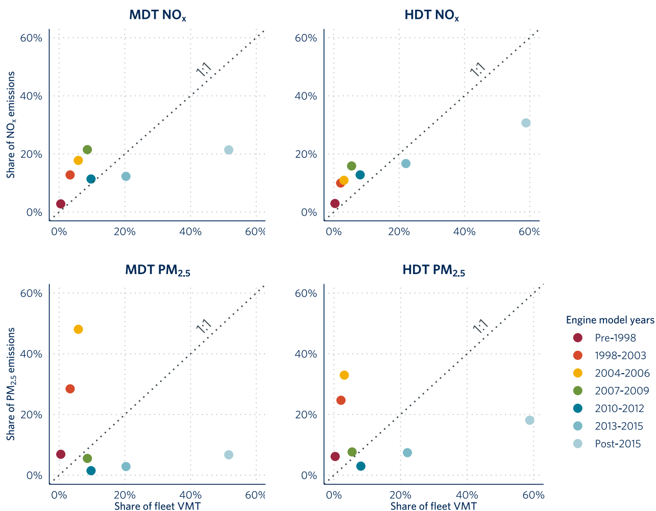
Figure 7. Share of emissions by engine model year (MY) group. Points above the line represent groups that contribute a disproportionate share of emissions.
