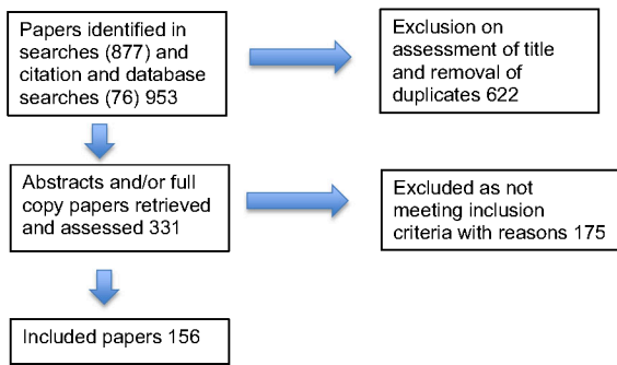
Fig. 1 Review flowchart
