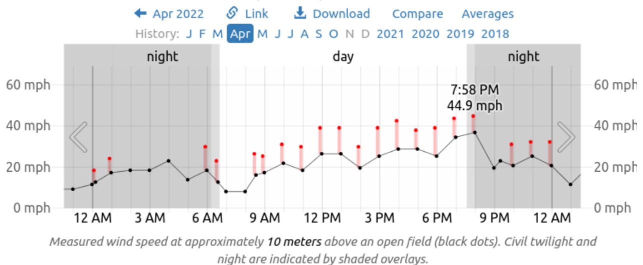
Wind Speed on Tuesday, April 12, 2022 at Holloman Air Force Base
