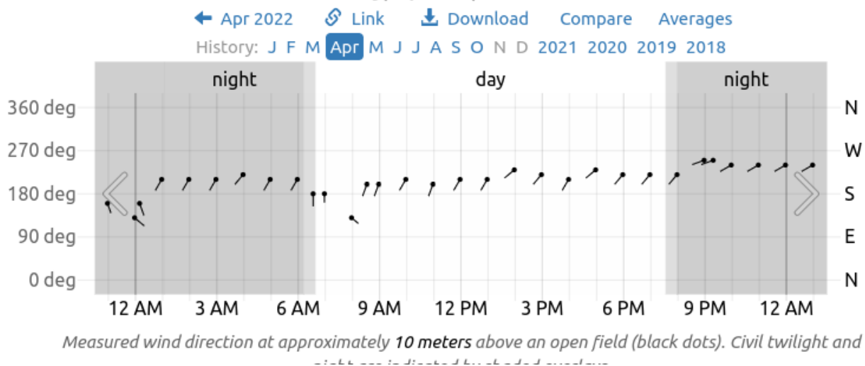
Wind Direction on Tuesday, April 12, 2022 at Holloman Air Force Base
