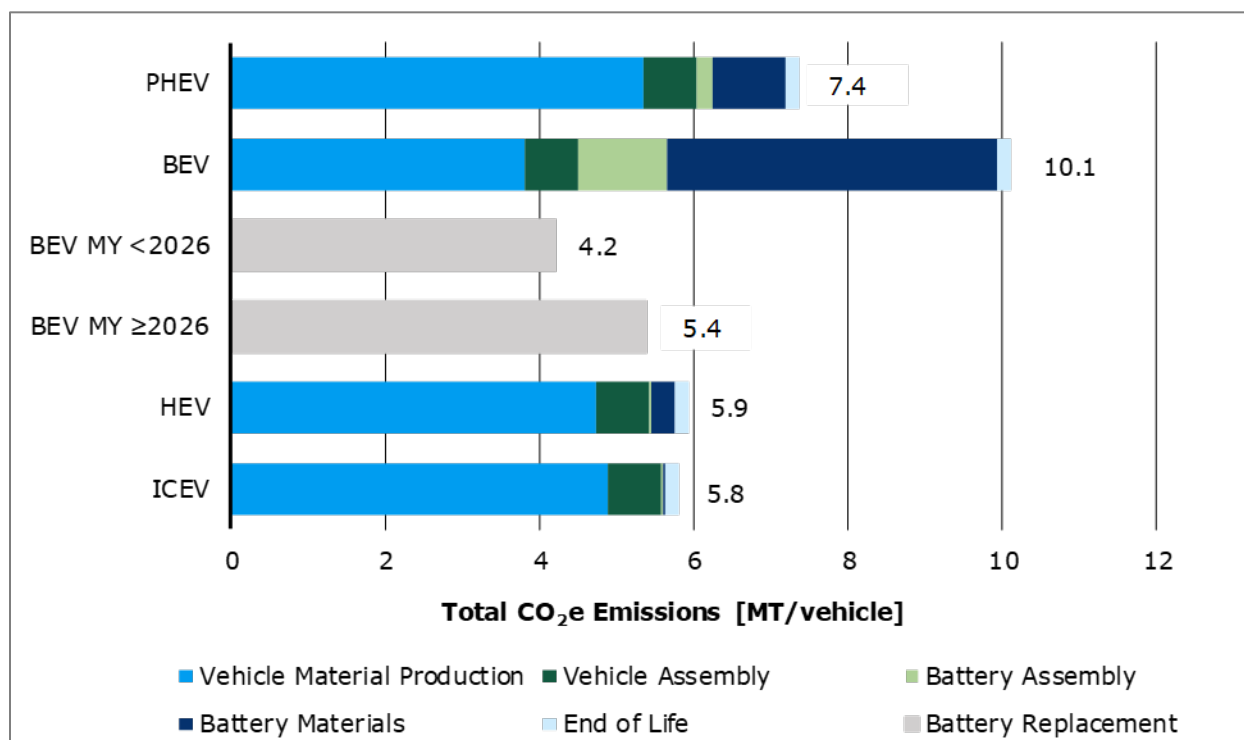
Figure 3-5: Vehicle Cycle and Battery Replacement GHG Emission Factors
