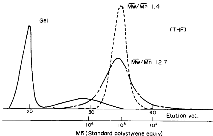
FIG. 8. Gel permeation chromatography (GPC) of iodo-regulated (IFKM, ----), isopentane-regulated ( \text{iso-C}_5\text{H}_{12} , - · - · -) and non-regulated (FKM, —) fluorocarbon elastomers in THF solvent. 38
