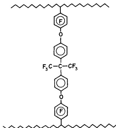
FIG. 29. The structure of the crosslinks formed after curing perfluorophenoxy-containing perfluoroelastomers with bisphenol AF. 72-74
