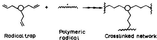
FIG. 16. The main reactions of the proposed crosslinking mechanism. 16
