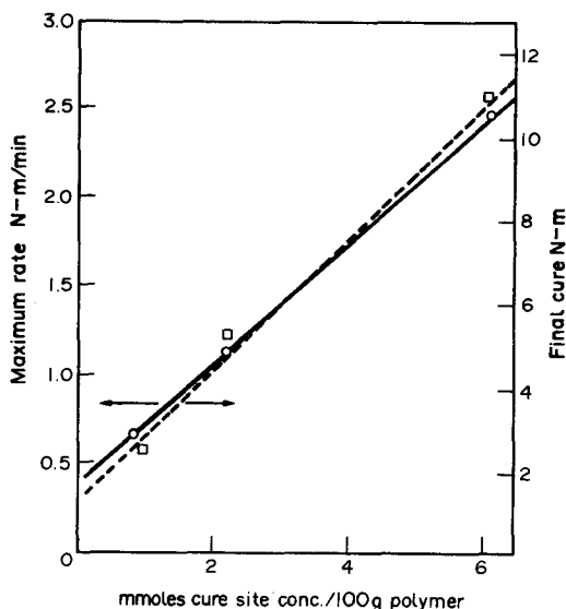
FIG. 14. The cure rate (open circles) and final cure state (squares) as obtained from ODR measurements at 177°C plotted as functions of cure site concentration. 16
