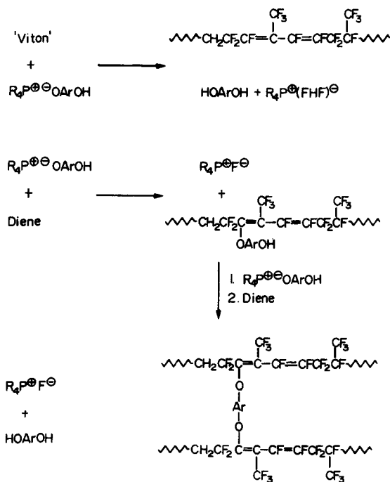
FIG. 13. Proposed scheme for crosslinking \text{VF}_2/\text{HFP} polymers with bisphenols in basic media. 17
