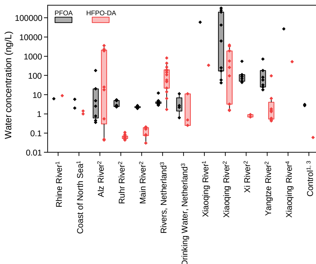
Figure 4. Concentrations of PFOA and HFPO-DA in rivers in Europe and China
