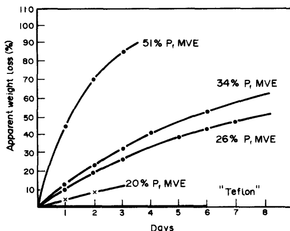
FIG. 26. Thermal stability of TFE/perfluoromethyl vinyl ether (P f MVE) in air in a glass vessel at 340°C. 69
