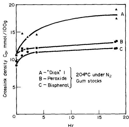
FIG. 17. The crosslink density of various cure systems plotted as a function of postcure time at 204°C under nitrogen. 16
