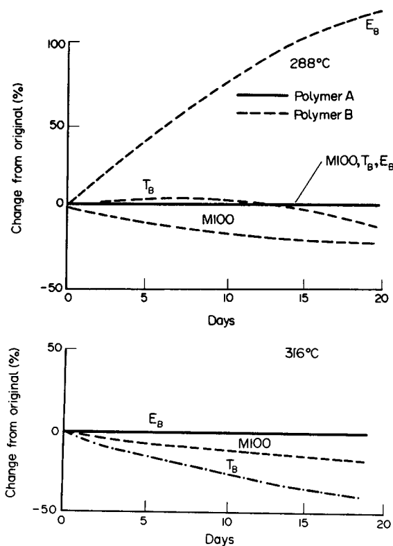
FIG. 34. Tensile properties after heat aging cured stocks of perfluoroelastomers: polymer A (nitrile-containing); polymer B (bisphenol AF cured); polymer C (halogen-containing, peroxide cured). 72 Footnotes as in Fig. 33.
