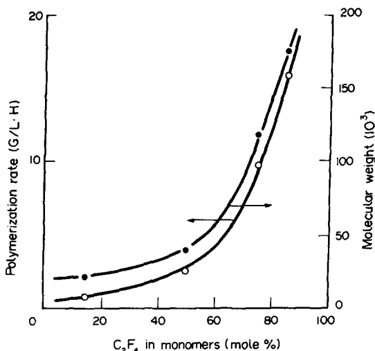
FIG. 20. TFE/propylene copolymers. Dependence of polymerization rate and molecular weight on the C_2F_4 fraction in monomers at 25°C. 39
