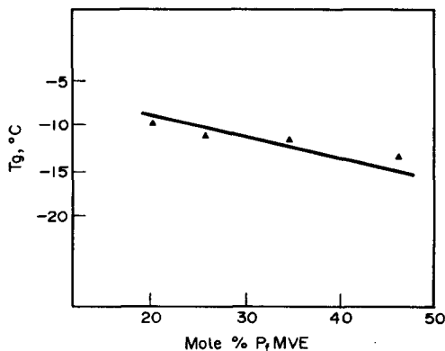
FIG. 25. T_g of TFE/perfluoromethyl vinyl ether (PFMVE) copolymers. 69
