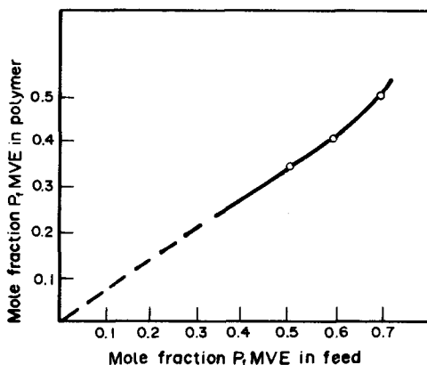
FIG. 24. TFE/perfluoromethyl vinyl ether (PFMVE) copolymers. Polymer composition as a function of monomer feed ratio at 60°C in an aqueous system at about 50% conversion. 69
