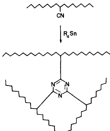
FIG. 31. The structure of the crosslinks formed after curing nitrile-containing perfluoroelastomers. 72-74
