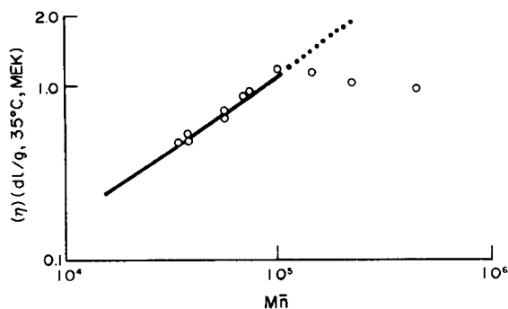
FIG. 6. Relationship between intrinsic viscosity ( \eta ) and number average molecular weight, M_n , of fluoroelastomers made in a semibatch polymerization system. 38
