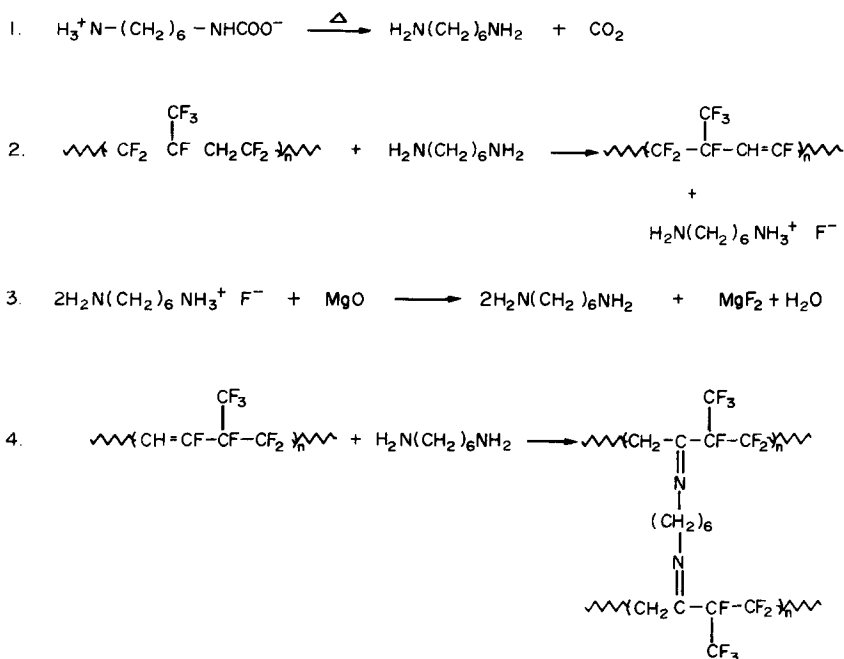
FIG. 10. Curing of vinylidene fluoride-containing fluoroelastomers with diamines. 14
