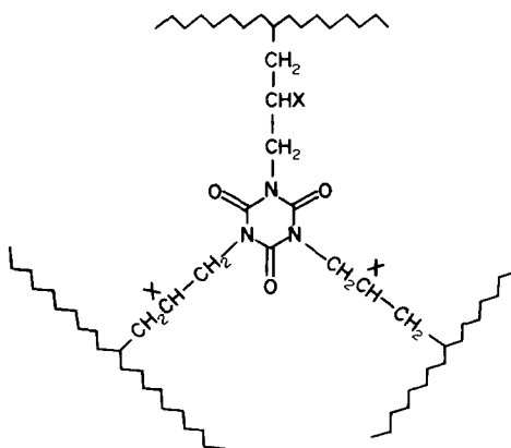
FIG. 32. The assumed structure of the crosslinks formed after curing of halogen-containing perfluoroelastomers with peroxides in the presence of a radical trap (triallyl isocyanurate). 72-74
