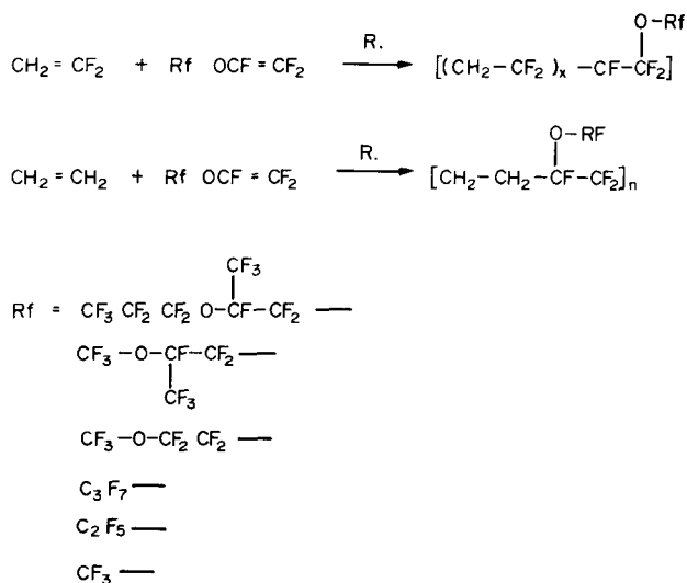
FIG. 9. Copolymers of perfluoroalkyl vinyl ethers with vinylidene fluoride (VF 2 ) and ethylene (E). 43,44 Terpolymers can also be made by adding tetrafluoroethylene (TFE) to the monomer mixture. 16,31–33,43,44
