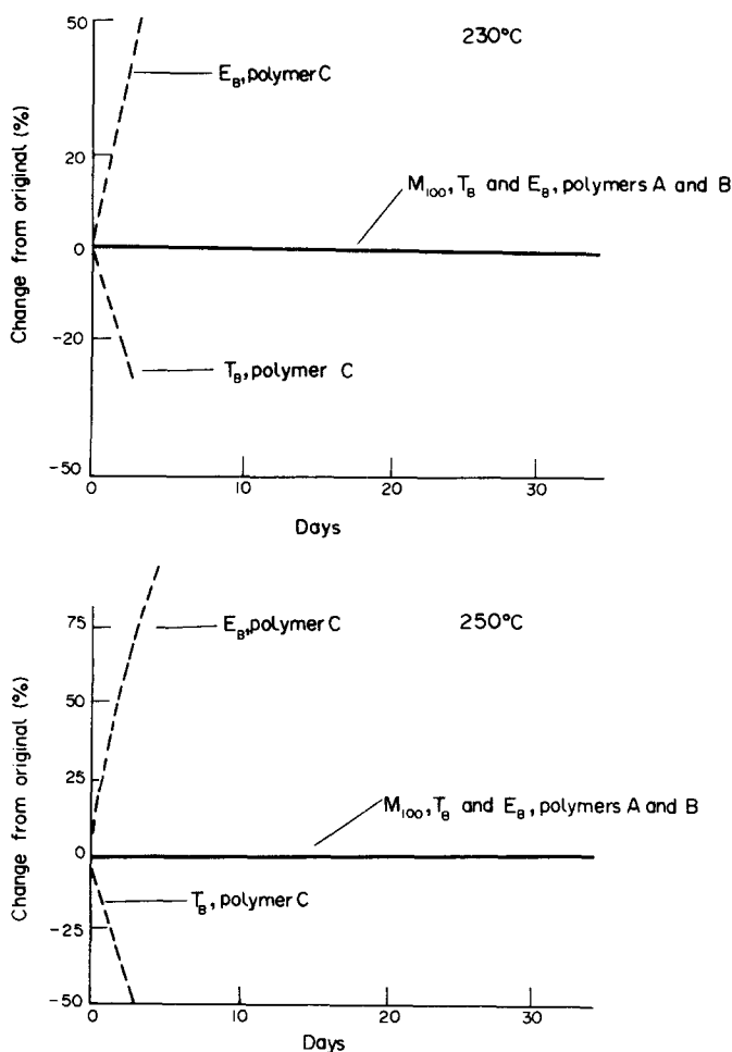
FIG. 33. Tensile properties after heat aging cured stocks of perfluoroelastomers: polymer A (nitrile-containing); polymer B (bisphenol AF cured); polymer C (halogen-containing, peroxide cured). 72 M_{100} = modulus at 100% strain; T_B = tensile strength at break; E_B = tensile elongation at break.
