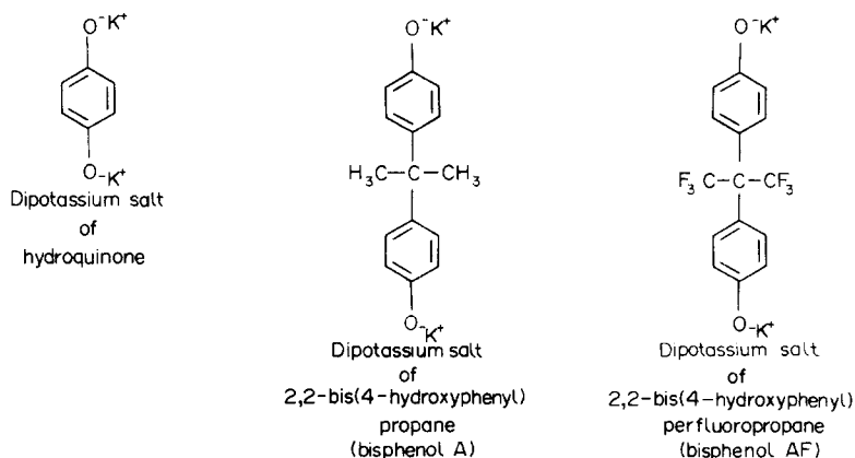
FIG. 28. Typical bisphenols dinucleophiles used in curing phenoxy-containing perfluoroelastomers. 70
