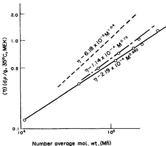
FIG. 7. Relationship between intrinsic viscosity ( \eta ) and mol. weight ( M_n ) for I(CF 2 ) 4 I regulated (—Δ—), C 4 F 9 I regulated (—O—) and non regulated (---) fluoroelastomers. 38
