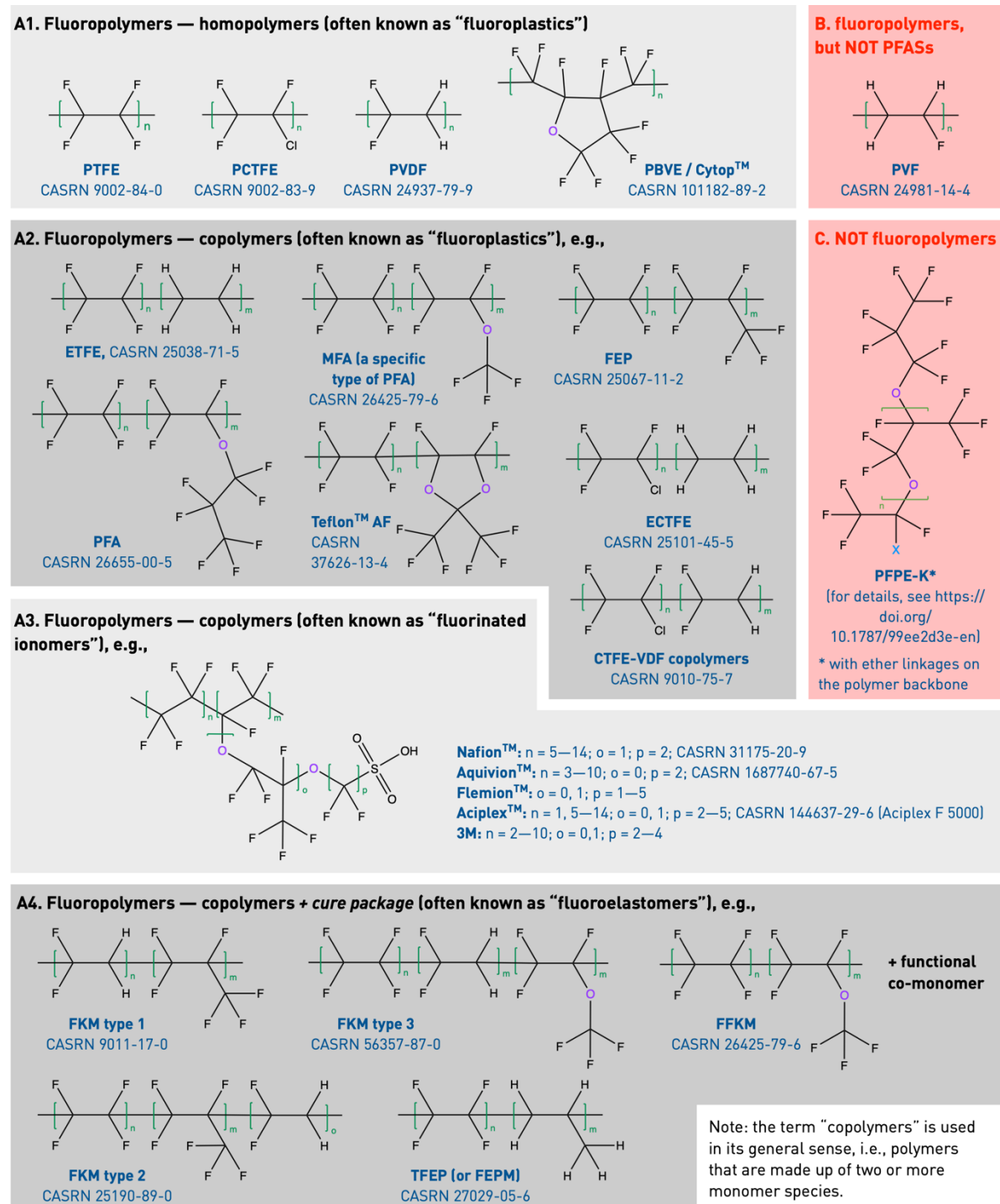
Figure 1. Examples of different types of fluoropolymers
