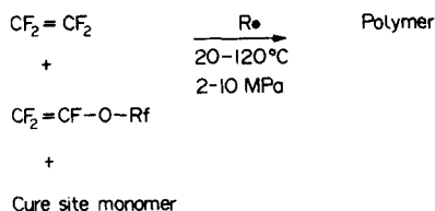
FIG. 23. Polymerization of perfluoroelastomers. 72-74
