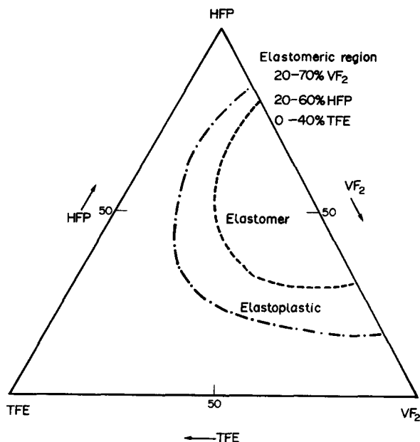
FIG. 3. Fluoroelastomeric compositions of polymers made from vinylidene fluoride ( \text{VF}_2 ), hexafluoropropylene (HFP) and tetrafluoroethylene (TFE). 7,8
