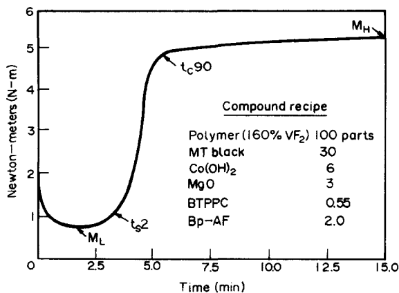
FIG. 11. Cure response by oscillating disc rheometry at 177°C of a compound optimized for use in O-rings. 17
