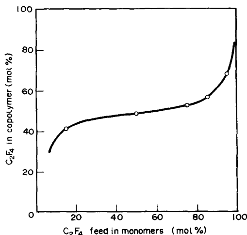
FIG. 19. Copolymerization curve of the TFE/propylene system. Polymerization in emulsion at 25°C and under 2.5 MPa pressure. 59
