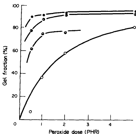
FIG. 21. Curing of TFE/propylene elastomers. Relation between peroxide level and gel fraction of an M_n 180,000 polymer; (O) without triallyl isocyanurate (TAIC); (●) with 3 phr TAIC; (⊖) with 2.4 phr divinylbenzene; (⊙) with 3 phr triallyl-cyanurate (TAC). 61
