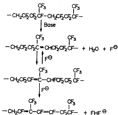
FIG. 12. Proposed reaction sequence of selectively base-sensitive site in \text{VF}_2/\text{HFP} polymers. 17
