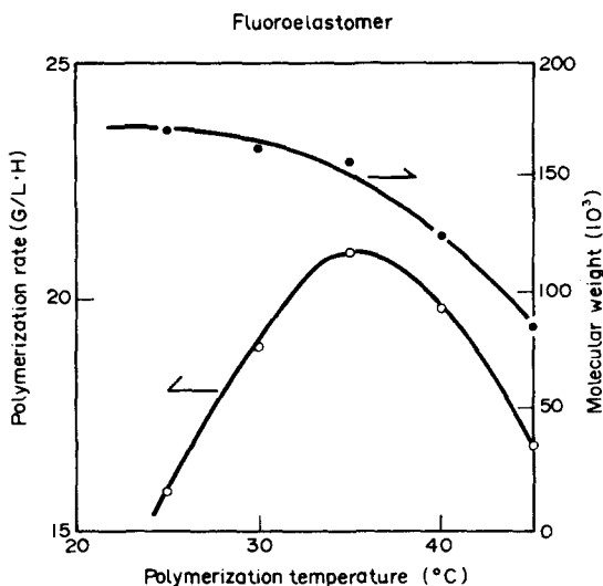
FIG. 18. TFE/propylene copolymers. Dependence of polymerization rate and molecular weight on polymerization temperature at TFE/ C_3H_6 (85:15) molar ratio of monomers. 59
