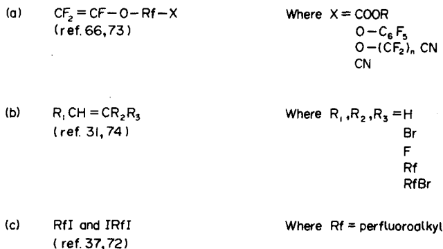
FIG. 22. Classes of cure site monomers as described in published articles and patents.
