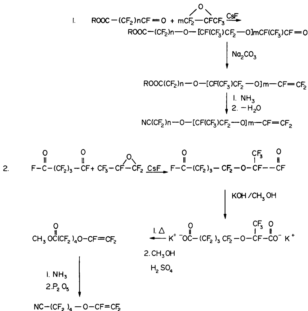
FIG. 30. Synthesis of perfluoro-(8-cyano-5-methyl-3,6-dioxo-1-octene) and perfluoro-(9-cyano-5-methyl-3,6-dioxo-1-nonene) where m = 1 and n = 2, 3 and perfluoro(4-cyanobutyl vinyl ether). 70,77
