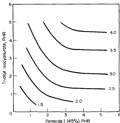
FIG. 15. Final cure state contours (N.m) as a function of peroxide (2,5-bis( t -butylperoxy) 2,5-dimethylhexane; 45% active ingredient) and coagent (triallyl isocyanurate) concentrations. 16
