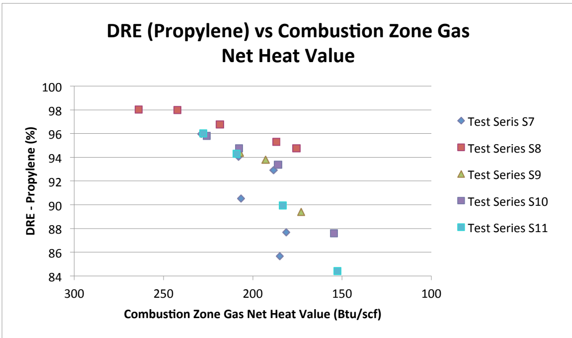
Figure 5-21b. DRE vs CZG NHV for Test Series S7, S8, S9, S10 and S11 (Note vertical axis DRE range = 84 to 100% and values on horizontal axis decrease from left to right)
